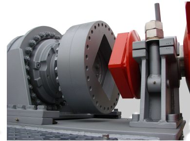
Hydraulically controlled coupling
